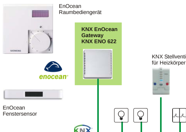
Fig. 5: Application example – heating control
